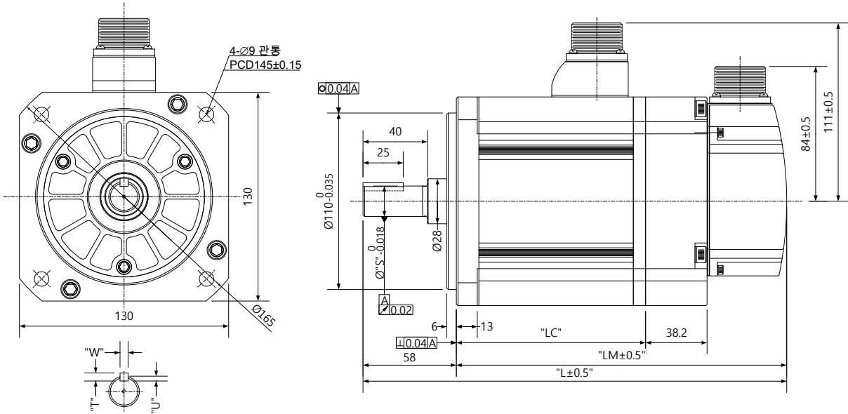
<Power Connector>
