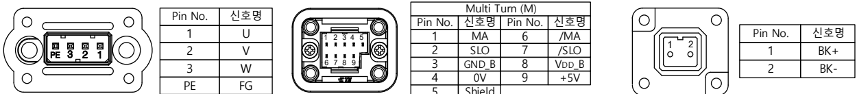
<Power Connector 핀 배열>
