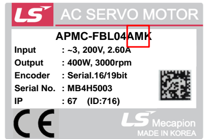
Absolute Multiturn(절대치멀티턴)
