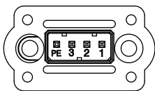
<Power Connector 핀 배열>
