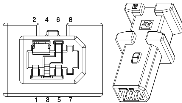
1971153-1(Tyco Electronics)
